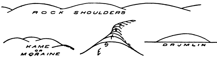
FIG. 345. — Character profiles referable to continental glacier.
